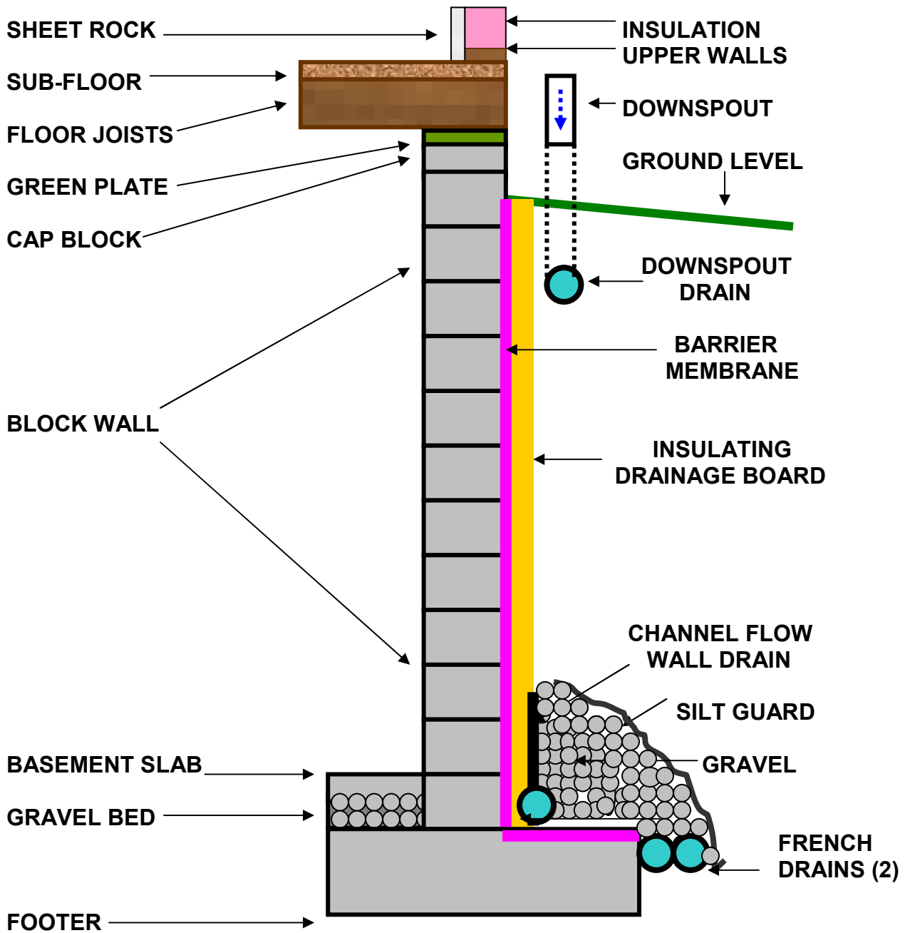
DUAL DAYLIGHT DRAINS WALL DRAIN & FOOTER DRAIN
